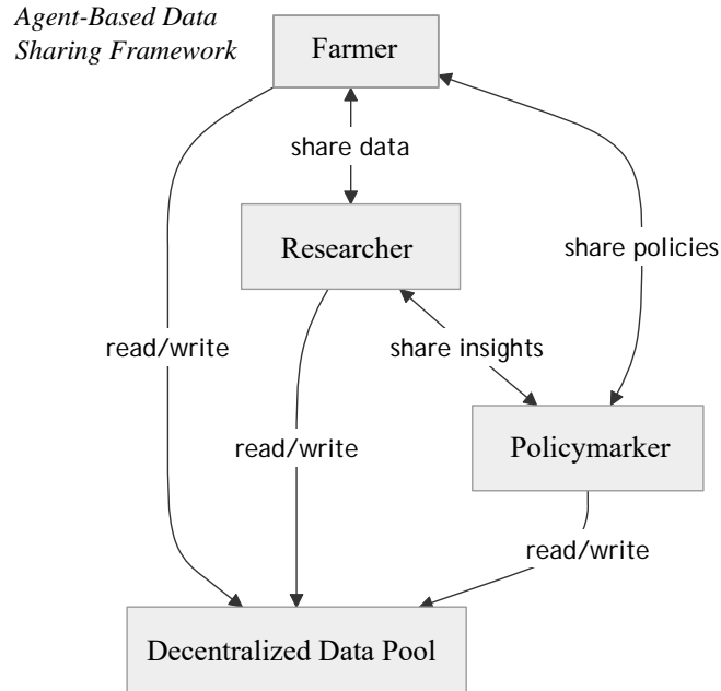
Figure 1. Interconnected Agricultural System with three agents - Farmer, Researcher, and Policymaker - sharing data and insights, all linked to a Decentralized Data Pool for data storage and access.
