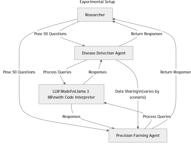
Figure 3. The diagram experimental setup involves two specialized agents: one for disease detection and another for precision farming recommendations. The agents interact with the Llama 3 8B model via the OpenAI Compatible API, utilizing a code interpreter tool for real-time data analysis.
