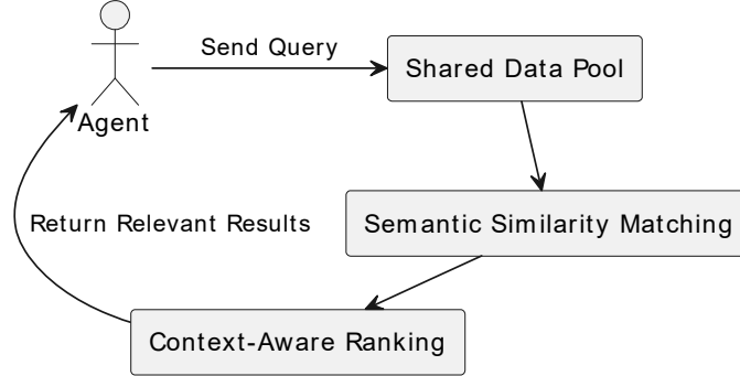
Figure 2. Agent interacting with a Shared Data Pool, The Shared Data Pool processes this question through a two-step retrieval process involving Semantic Similarity Matching and Ranking Algorithms with Context.
