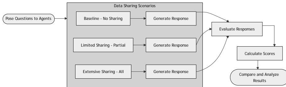
Figure 4. Evaluation Process of Agent Responses
